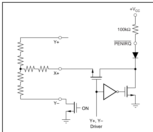
FIGURE 15. \overline{\text{PENIRQ}} Functional Block Diagram.
