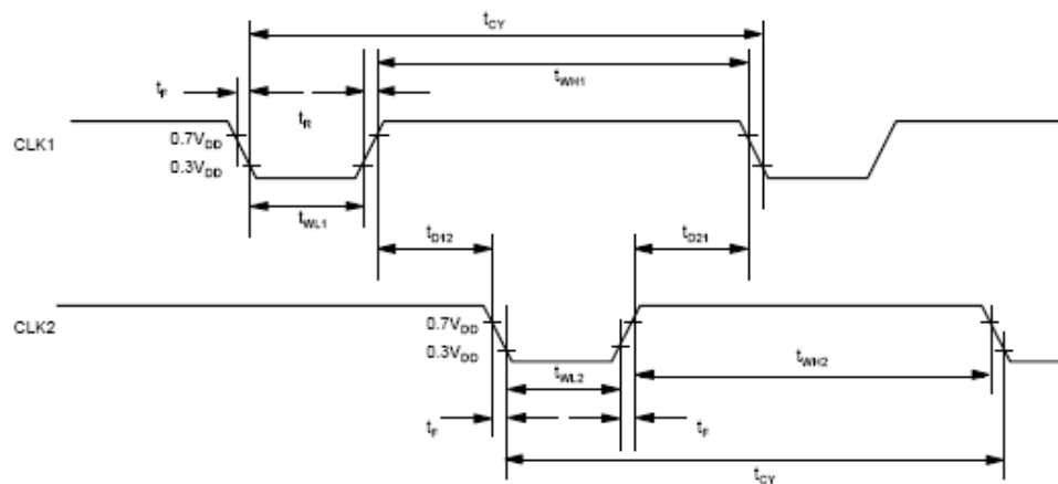
Figure 1. External clock waveform
